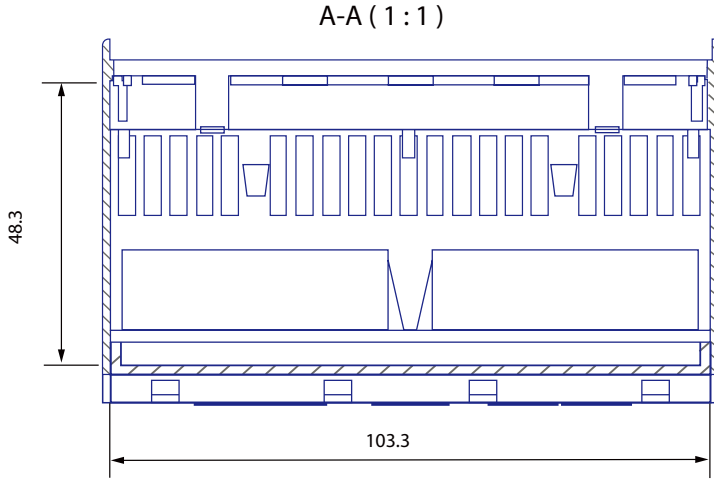
Figure 3: Front view
