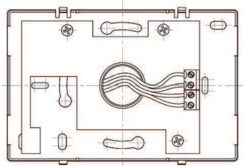
Fig. 7. The way of assembly electrical cords
