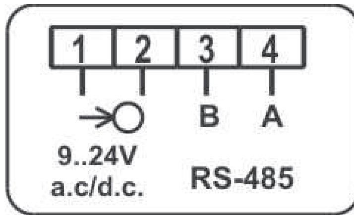
Fig. 5. Way of electrical signal connection
