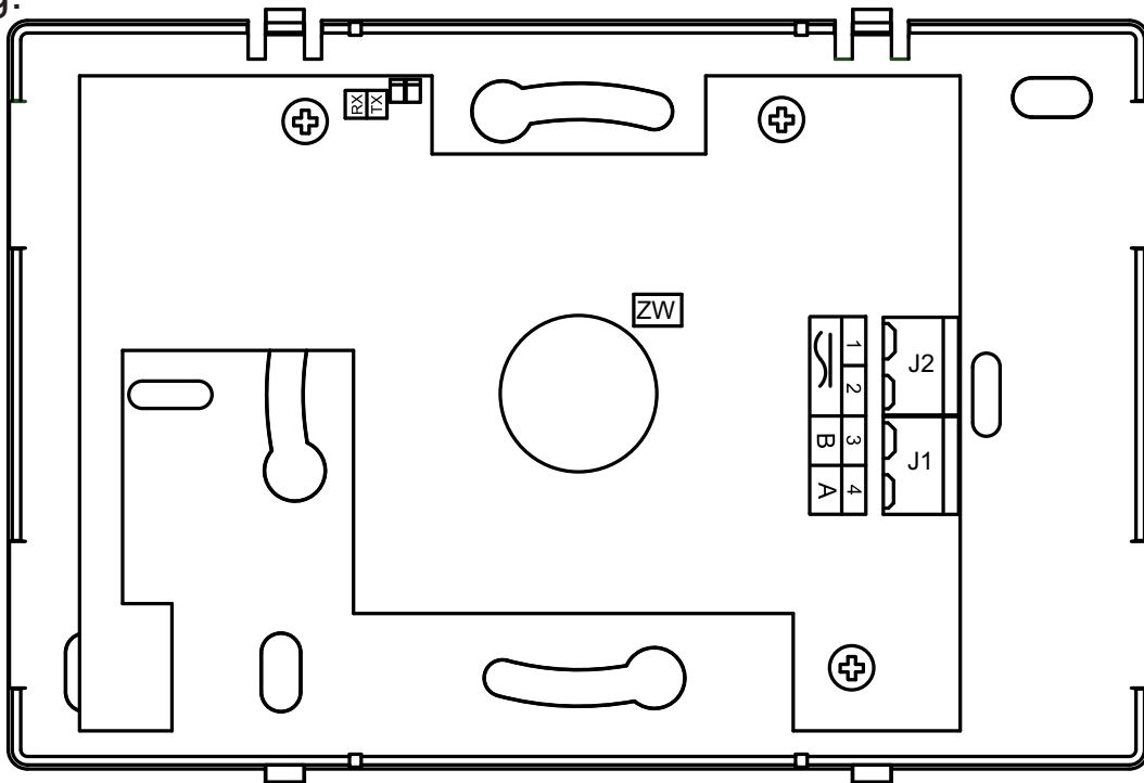
Fig 4. Marking of terminals for the connection of external signals
